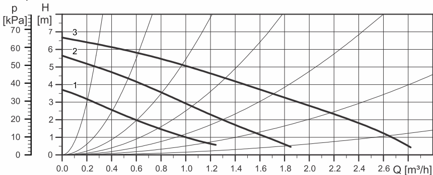
Pump available head of 32/40kW boiler
