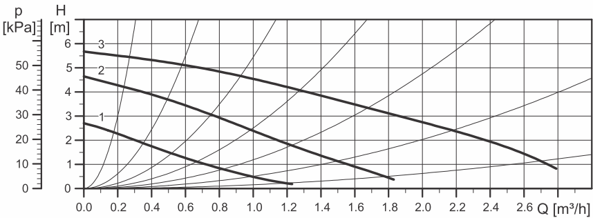
Pump available head of 32/40kW boiler
